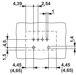
Drilling diagram
