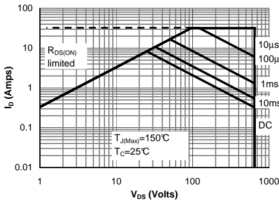
Figure 9: Maximum Forward Biased Safe Operating Area for AOT8N65 (Note F)
