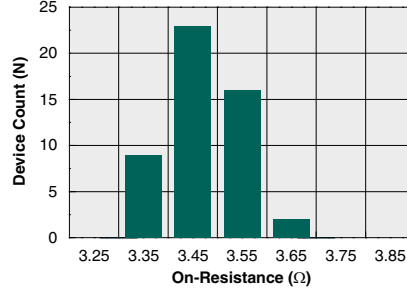
Typical On-Resistance Distribution (N=50, I_F=5\text{mA} , I_L=500\text{mA} , T_A=25^\circ\text{C} )
