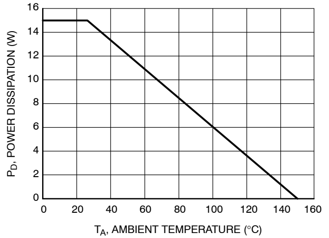
Figure 8. Power Derating
