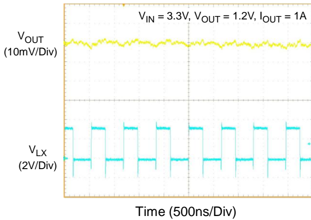
Voltage Ripple
