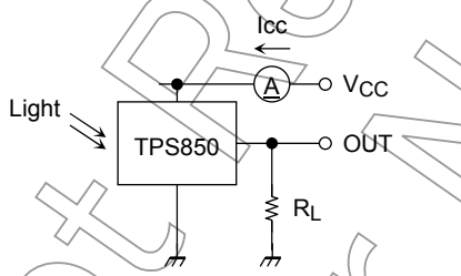
Figure 3 Consumption current measurement circuit
