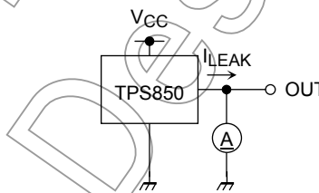
Figure 2 Dark current measurement circuit
