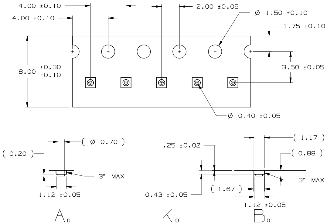
Figure 13. Pocket tape dimensions for LUXEON UV FC1.
