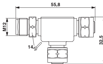
M12 T-distributor
